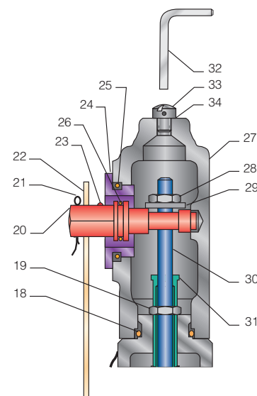
PACKED LEVER (shown with gag option)
