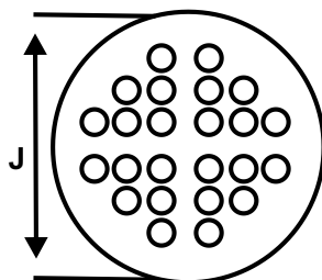
4-Pass Tubesheet without Bolt Holes
