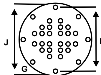
Tubesheet with Bolt Holes
