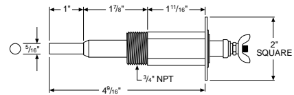
EL1214-P - 3/4" NPT
